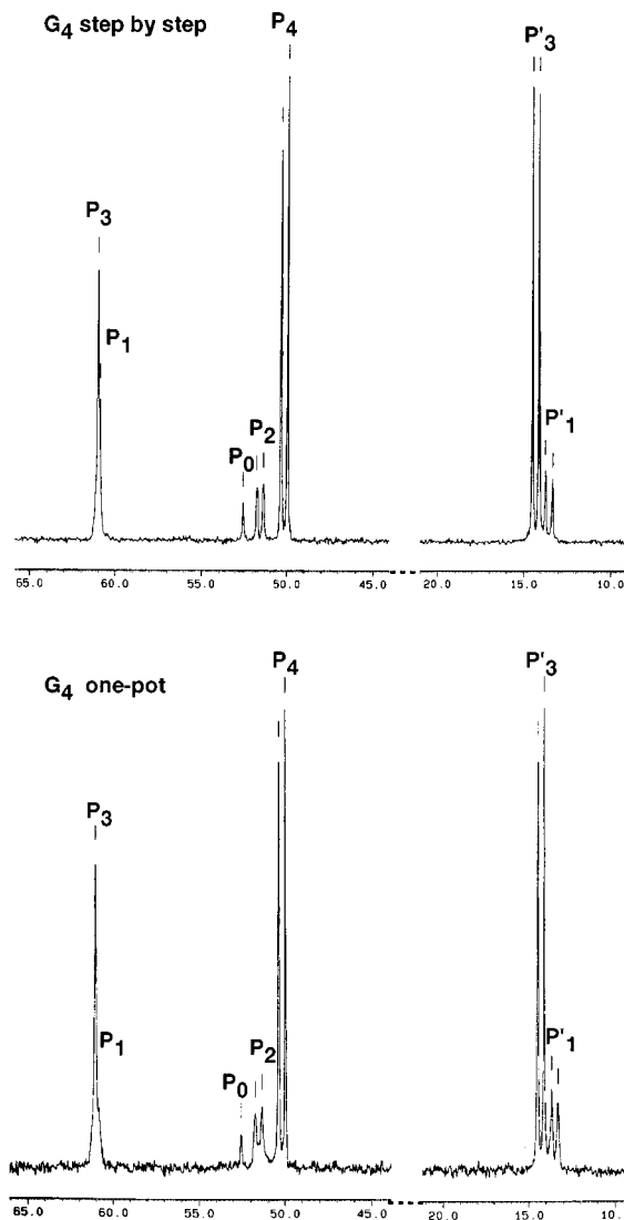
Figure 1. 31 P spectra of dendrimers G4 step-by-step and G4 one-pot.
